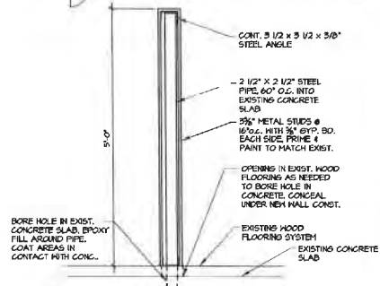
3 TYPICAL 60" PARTITION SCALE: 1"=1'-0"
