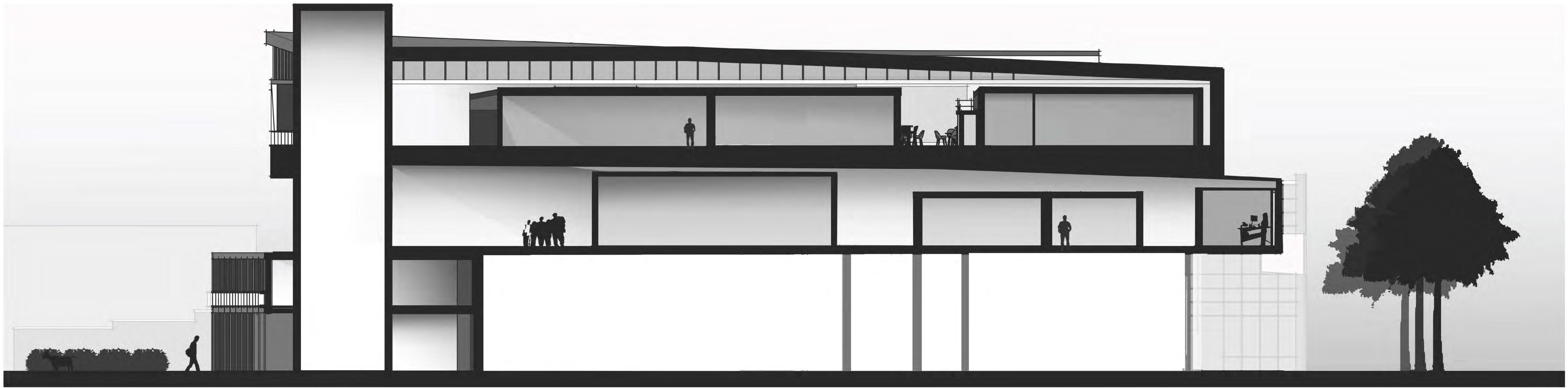
East-West Section
