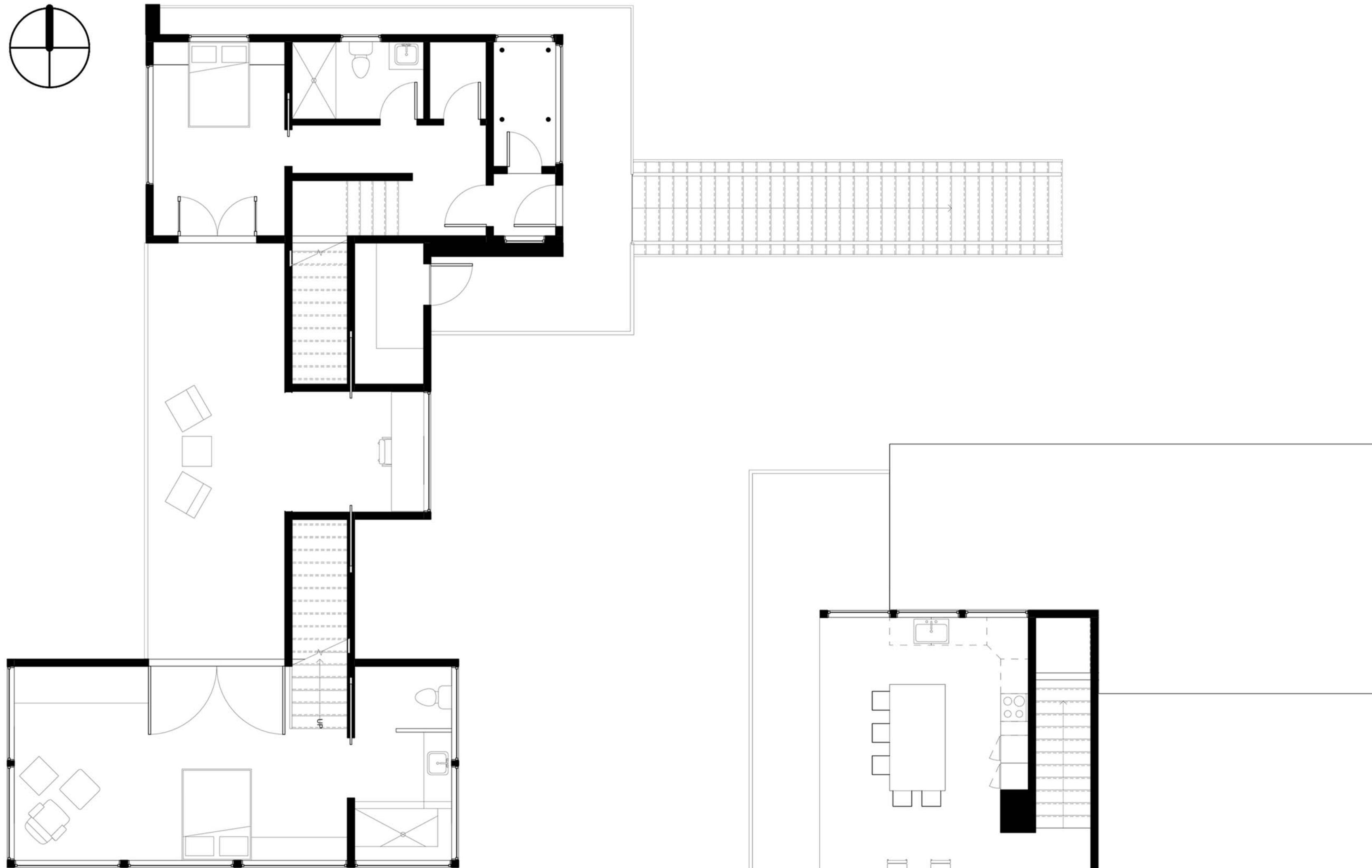
FIRST FLOOR
