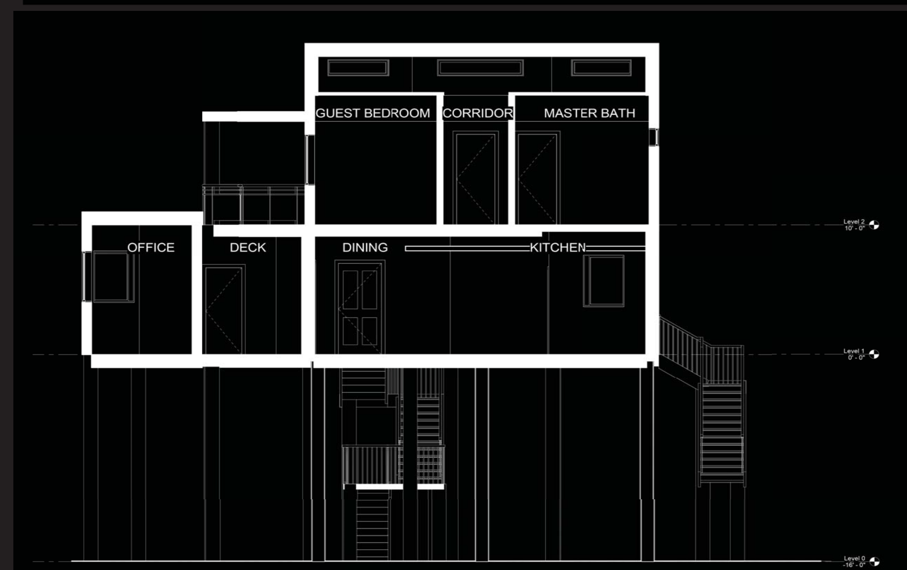
CROSS SECTION
